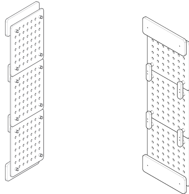
C WALL UNIT BACK VIEW not to scale
