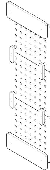
C WALL UNIT BACK VIEW not to scale
